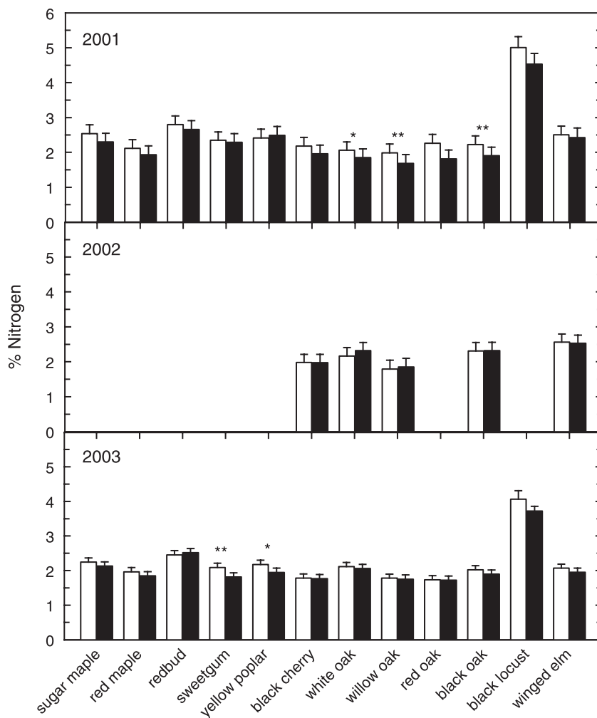
Fig. 2 Effects of elevated CO 2 on leaf nitrogen concentration (% dry mass) for plants grown under ambient (c. 386 \mu\text{l l}^{-1} ) and elevated (c. 586 \mu\text{l l}^{-1} ) CO 2 for each of the three years. Columns represent the least-squared means ( \pm 1 SE) of the three ambient and three elevated CO 2 plots (open columns, ambient CO 2 ; closed columns, elevated CO 2 ). Within a species and year, statistical significance of pairwise comparisons is indicated above columns (* P < 0.1 , ** P < 0.05 , *** P < 0.01 ).
