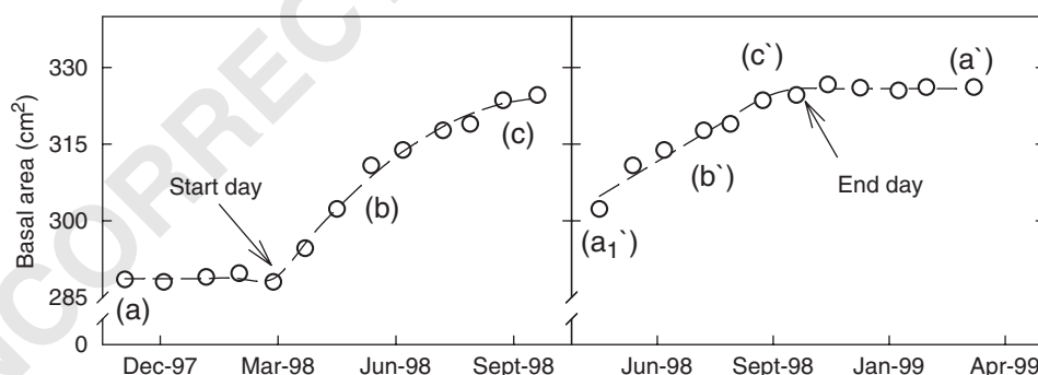
Fig. 1 Basal area (BA) for a typical Pinus taeda tree from December 1997 through April 1999. BA was calculated from measurement of bole circumference. The symbols represent measured values and the lines represent functions fit to the data. Two functions were used to describe the progression of growth from winter into summer and autumn (left panel). In winter, BA (basal area) = a (constant), and during summer and autumn, BA = a + b(\text{day}) + c(\text{day}^2) ; where b is the initial increase in tree size and c is the curvature of growth late in the season. The intersection of these two functions defined the 'start day'. The progression of growth from summer into the following winter was also described by two functions (right panel). During summer and autumn, BA = a_1' + b'(\text{day}) + c'(\text{day}^2) and during the following winter, BA = a_1' . The intersection of these two functions defined the 'end day'. The 'end day' was then modified to accommodate the gradual cessation of growth late in the year (see methods).
