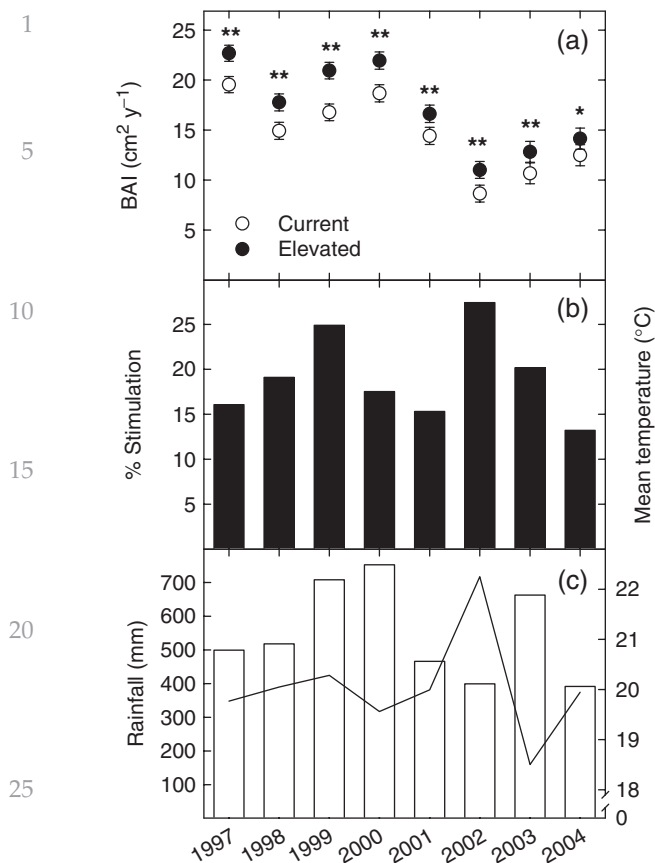
Fig. 3 The basal area increment (BAI) for Pinus taeda trees exposed to ambient \text{CO}_2 (○) and elevated \text{CO}_2 (●) (a) and the percentage stimulation in BAI caused by elevated \text{CO}_2 (b) and the variation in total rainfall (open bars; mm) and mean temperature (black line; ^{\circ}\text{C} ) during the active growth period (c). Symbols in panel a are least square means from three independent replicate forest plots. Error bars represent \pm 1 standard error of the difference between LS means. Treatment differences at P < 0.1 and P < 0.05 , indicated by '*' and '**', respectively, were estimated using upper level linear contrast statements within a repeated measures mixed model ANOVA (Table 1).
