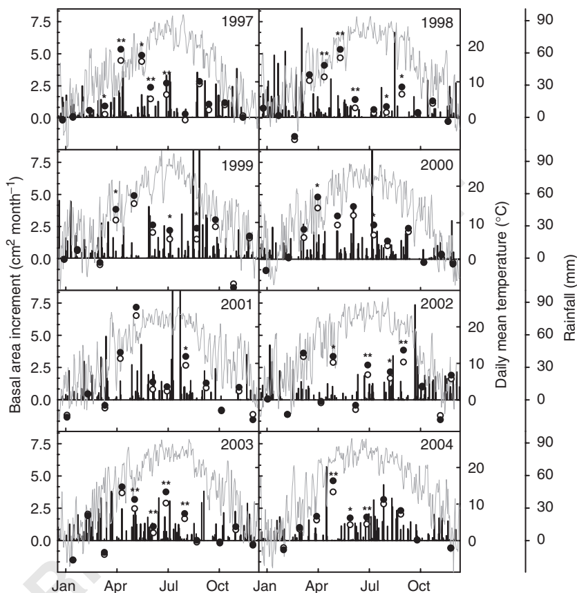
Fig. 2 Mean monthly basal area increment (cm month -1 ), mean daily temperature (grey line; °C) and daily rainfall (black bars; mm) for each year of the experiment. Basal area increment of Pinus taeda exposed to ambient CO 2 is represented by 'o' and elevated CO 2 is shown by '•'. Symbols for monthly BAI represent least square means from three independent replicate forest plots. Treatment differences at P<0.1 and P<0.05, indicated by '*' and '**', respectively, were estimated using upper level linear contrast statements within a repeated measures mixed model ANOVA conducted within each year 1997 to 2004.
