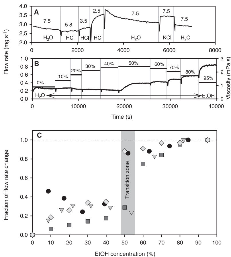
Fig. 3. Demonstration that hydrogels are responsible for ion-mediated flow enhancement in stems of L. nobilis . (A) Effect of pH on flow rate. Numbers above the curves indicate the solution pH. (B) Effect of nonpolar solvent on flow rate through stem segments maintained at 25°C. Percentages indicate the % ethanol concentration of the perfusing solution. Horizontal bars indicate solution viscosity. (C) Relative change in flow rate as a function of ethanol concentration. Flow rates were adjusted for viscosity ( \eta ) by multiplying flow rates by \eta_{\text{solution}}/\eta_{\text{water}} (35). Symbols represent different stem segments. Measurements were scaled so that the maximum difference in flow rate = 1. In all cases, there was a marked increase in flow rate at \sim 50\% ethanol.
