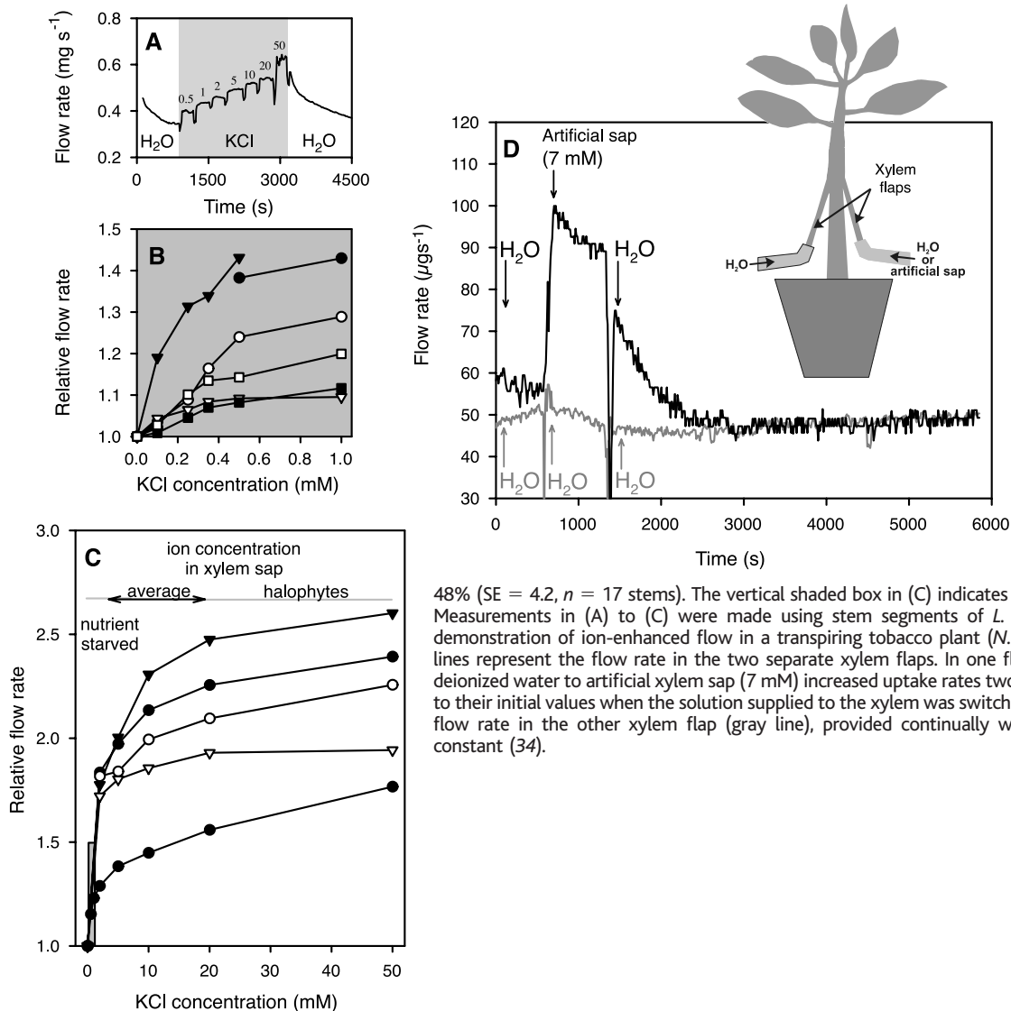
Fig. 1. Effect of KCl concentration on flow rate through xylem. (A) Time course of typical experiment showing a slow decline in flow rates with deionized water and increasing flow rates with KCl. Numbers above the curves indicate KCl concentration (mM). Sharp drops in flow rate between consecutive treatments reflect temporary pressure drops associated with switching between solutions. (B and C) Relative flow rate (flow rate with indicated solution/flow rate with deionized water) as a function of KCl concentration (0 to 1 mM and 0 to 50 mM, respectively). Symbols represent different stem segments. The average increase in flow rate in response to 10 mM KCl was
