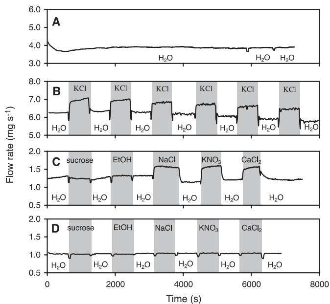
Fig. 2. Effect of solution composition on flow enhancement. Measurements were repeated with qualitatively consistent results for five different L. nobilis stem segments; a representative set of measurements is shown here (33). (A) Sustained perfusion of deionized water. Switching between deionized water containers does not alter the flow rate. (B) Effect of repeated changes between deionized water and KCl solution (10 mM). (C) Effects of solution composition (10 mM) on flow rate through stem segments. EtOH, ethanol. (D) Effects of solution composition (10 mM) on flow rate through a 74-cm-long plastic capillary tube (polyetheretherketone, 64 \mu\text{m} in diameter).
