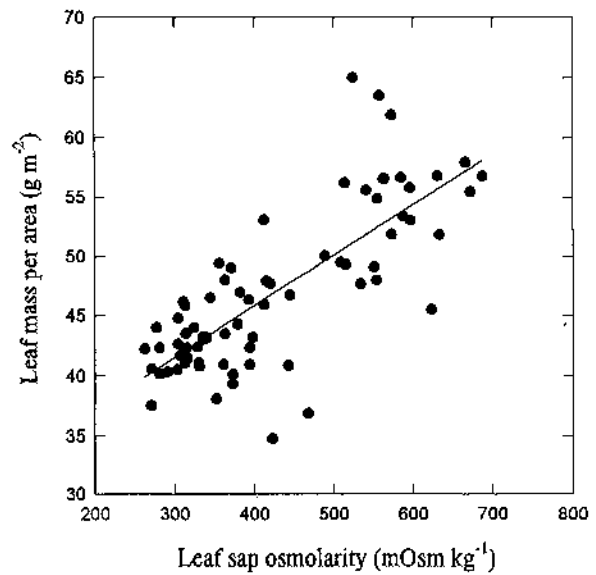
Fig. 4 Leaf mass per area (specific leaf mass) as a function of leaf sap osmolarity for Scaevola sericea grown under different salinity treatments ( r^2 = 0.59 ).
