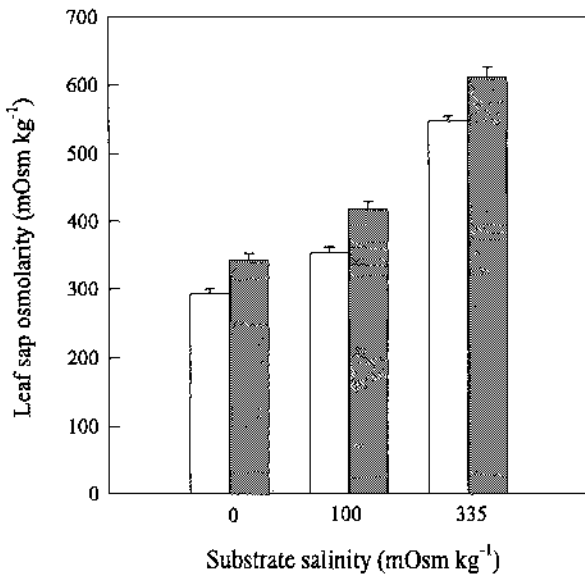
Fig. 2 Leaf sap osmolarity as a function of substrate salinity for Scaevola sericea exposed to spray with 0 (open bars) and 1200 mg m -2 d -1 (dashed bars) of sea water salt. The segments on each bar indicate one SE above the mean.
